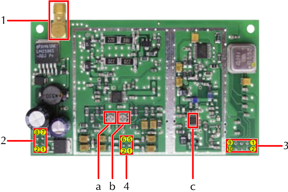
board dimensions: 60×100 mm
